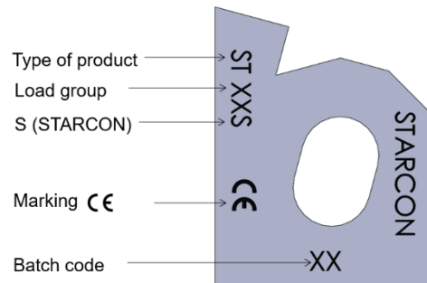
Figure 2 Marking on top of the STA ST
