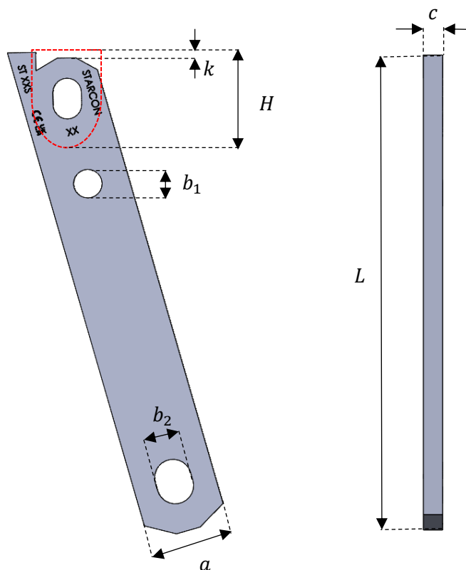
Figure 12 STA ST sketch.
