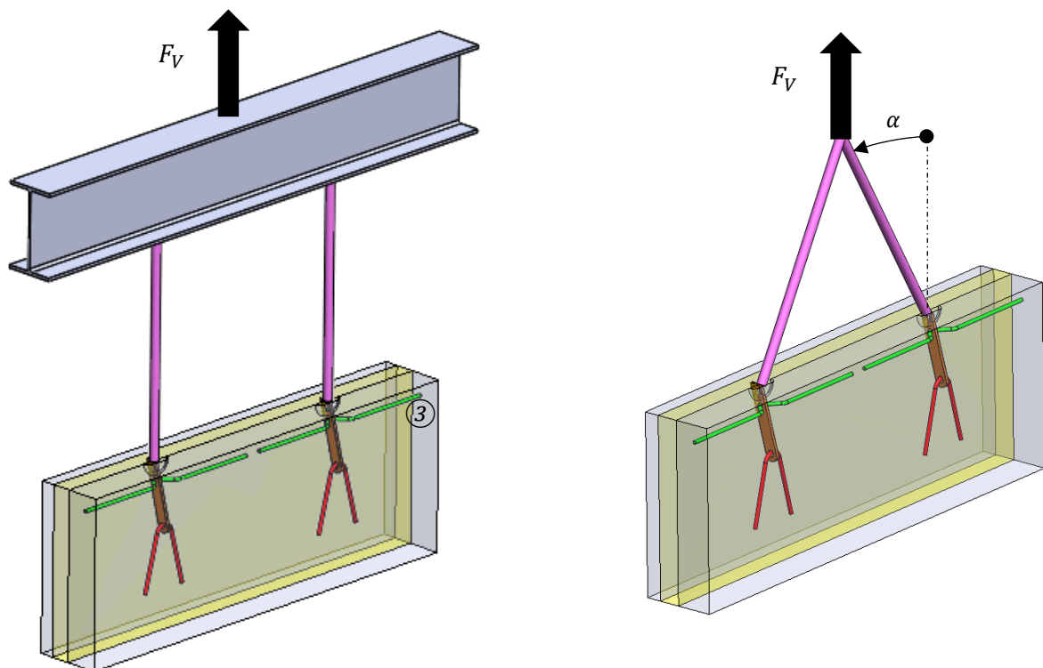
Figure 11 STA ST lifting recommendations illustration.
