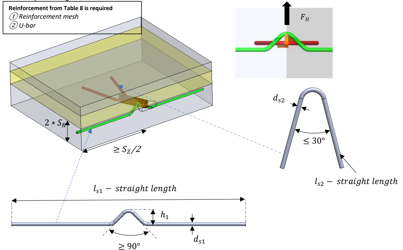
Figure 10 Reinforcement requirements for tilting and turning of the element.
