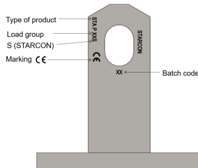
Figure 2 Marking on top of the STA P.
