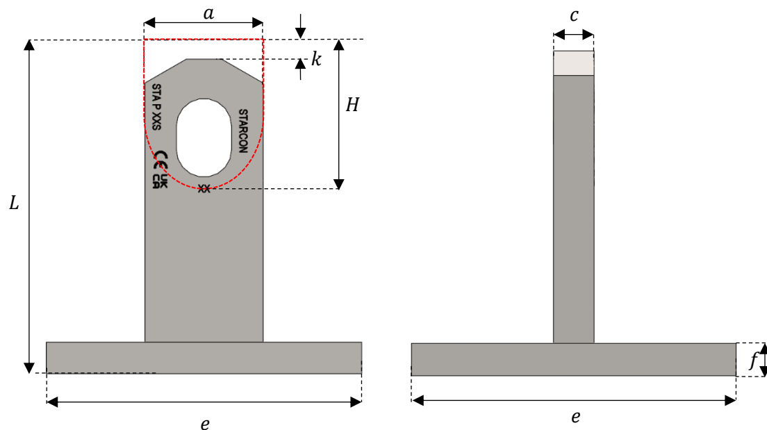
Figure 10 STA P sketch.
