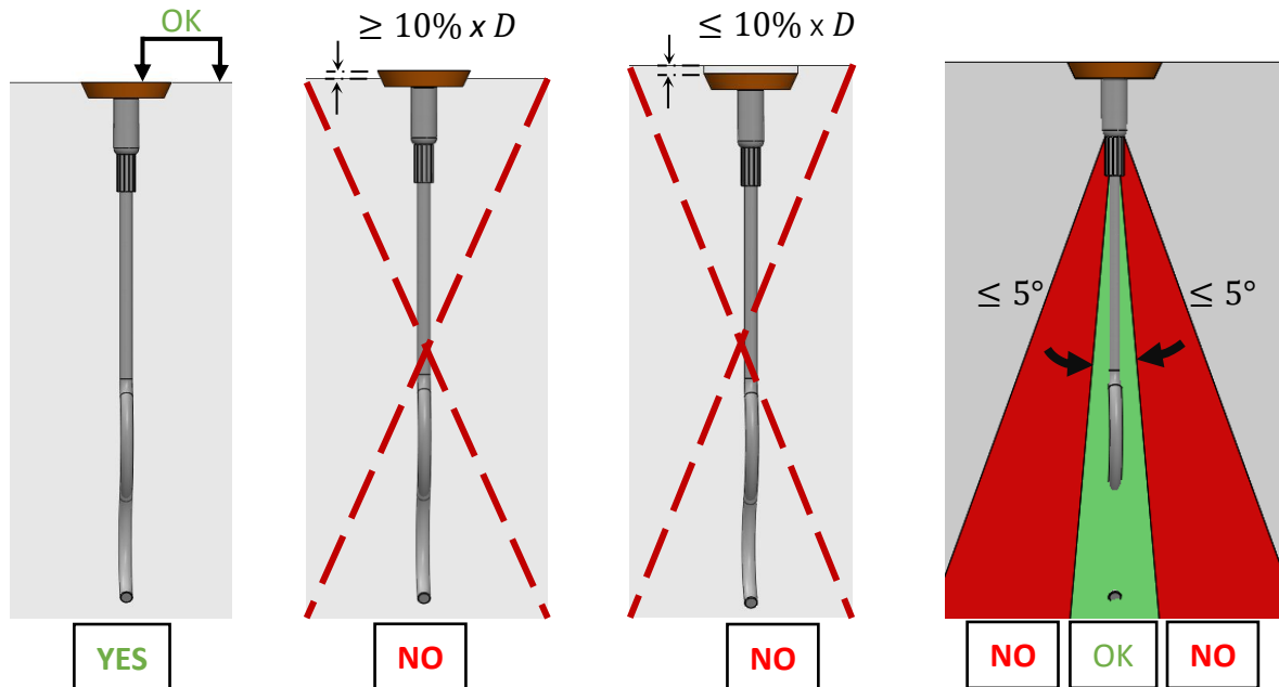
Figure 4 Correct placement of nailing plate.
