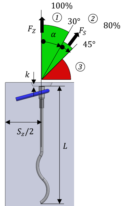
Axial & Diagonal pull lifting
