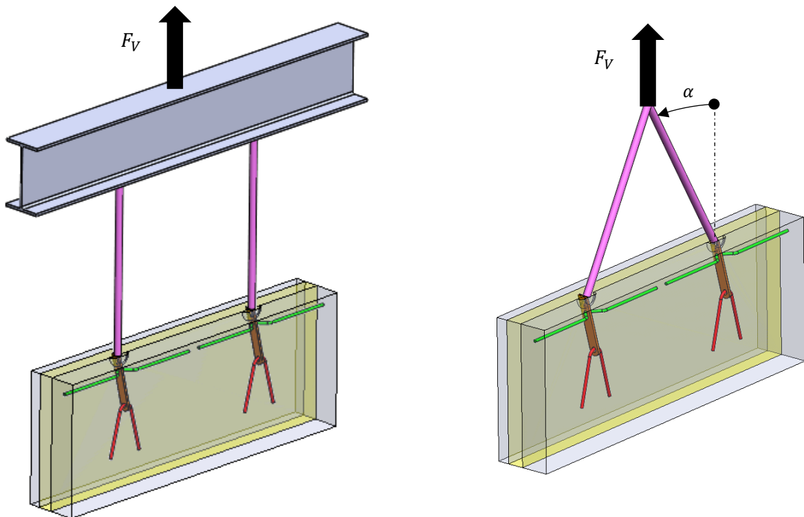
Figur 11 STA ST løfteanbefalinger, illustration.
