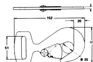
Palkrog type PA5 Latch hook type PA5
