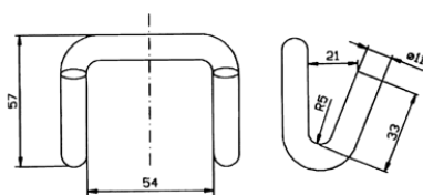
U-krog type U11 U-hook type U11
